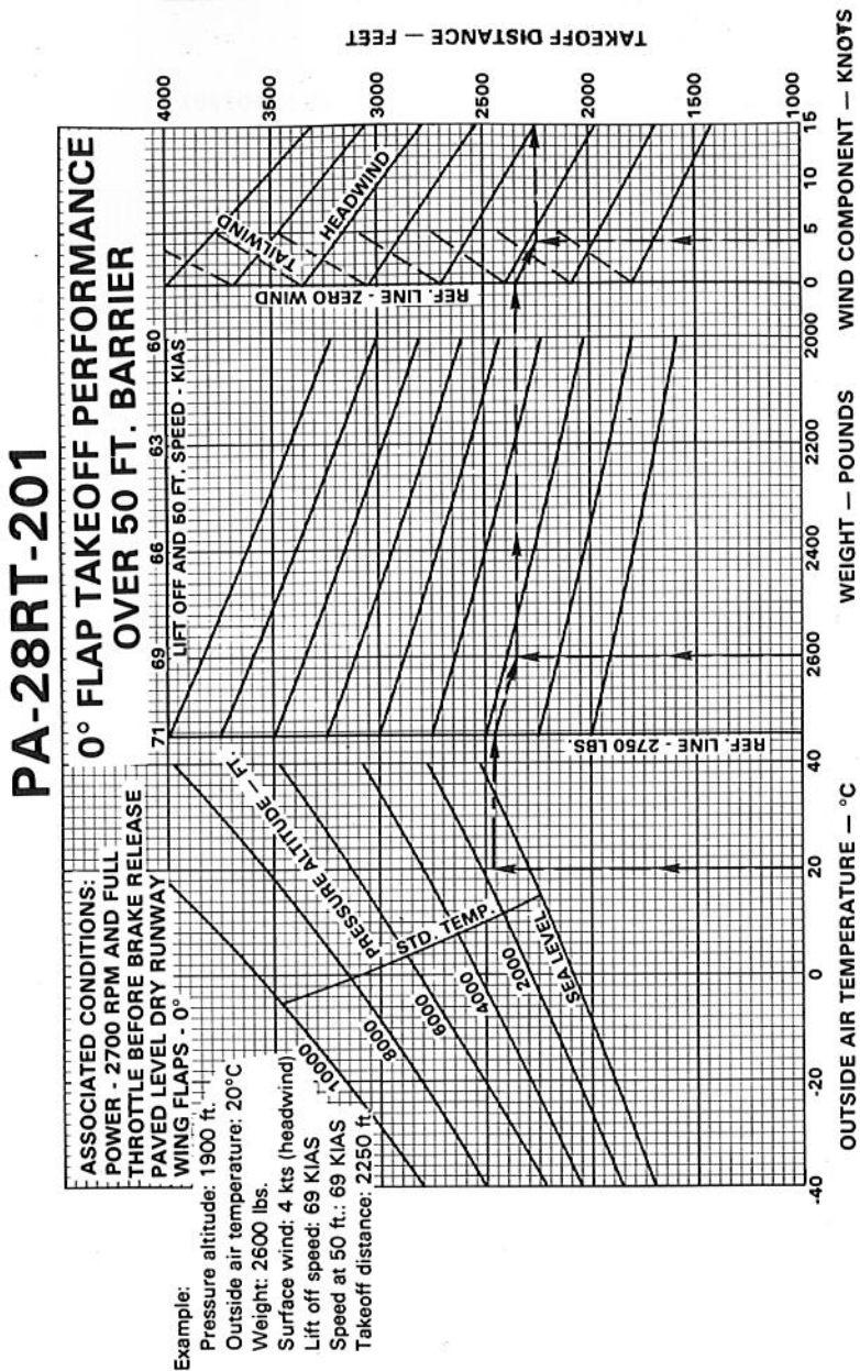
0° FLAP TAKEOFF PERFORMANCE
