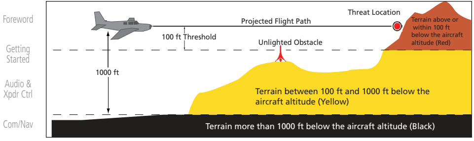
Figure 11-6 Terrain Altitude/Color Correlation
