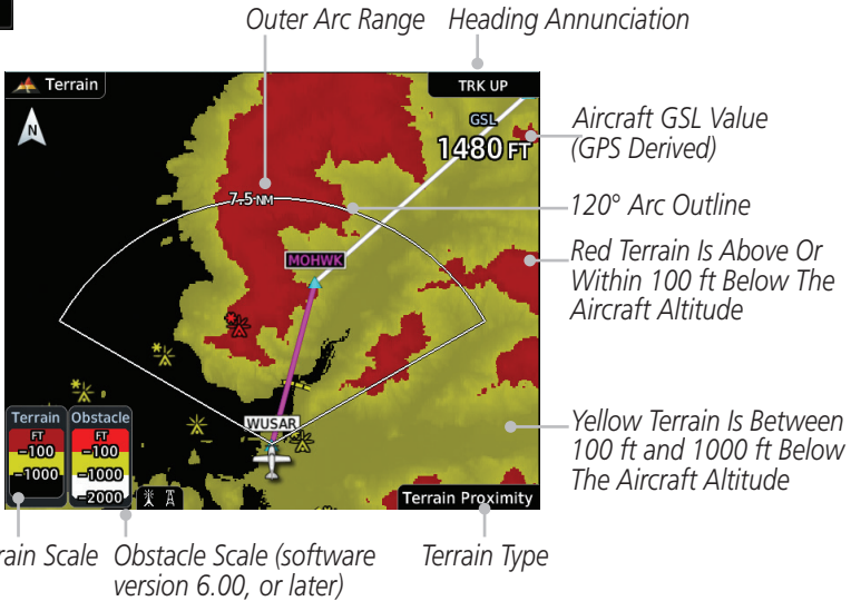
Figure 11-4 Terrain 120° Arc View
