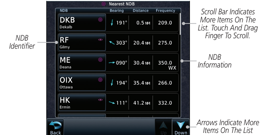
Figure 13-13 Nearest NDB
