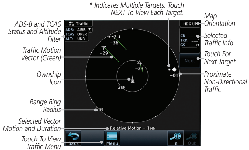
Figure 10-14 Relative Motion (Green Vectors)
