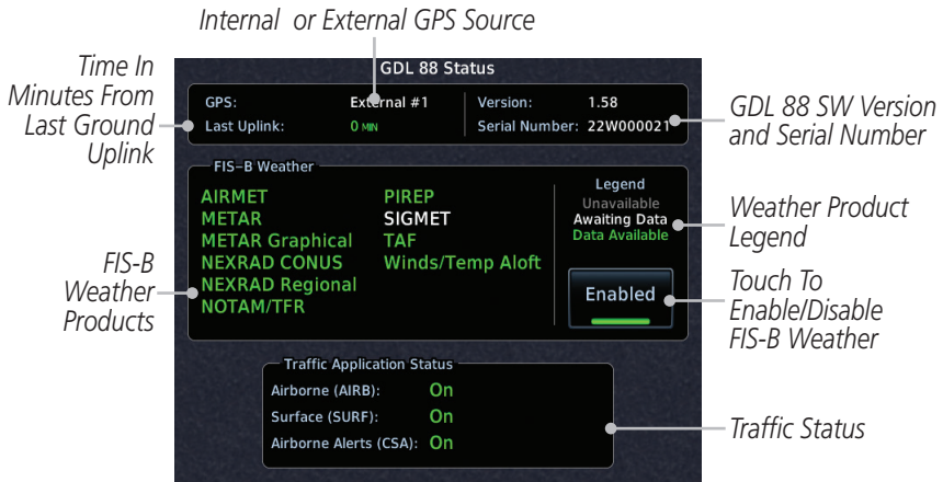
Figure 16-13 GDL 88 Status
