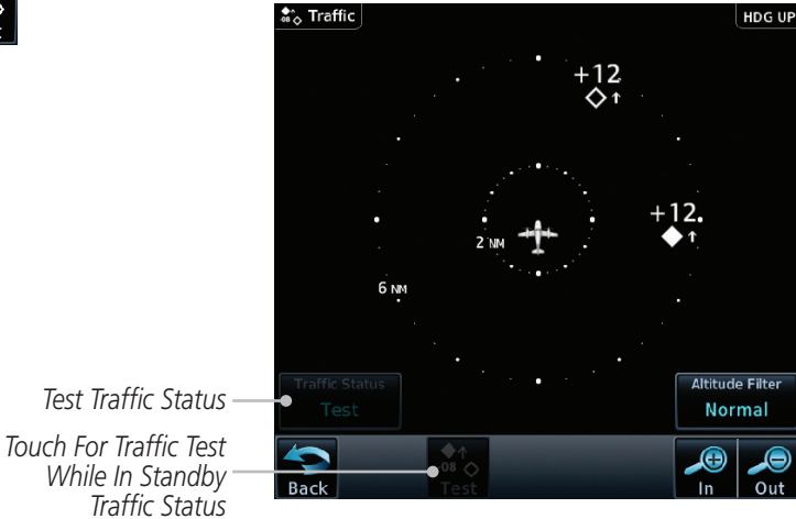
Figure 10-2 Traffic Test Mode
