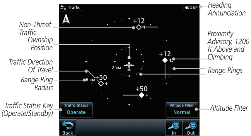
Figure 10-5 Traffic Page
