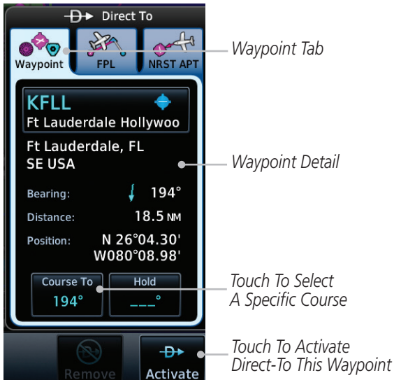
Figure 5-3 Direct-To Selection
