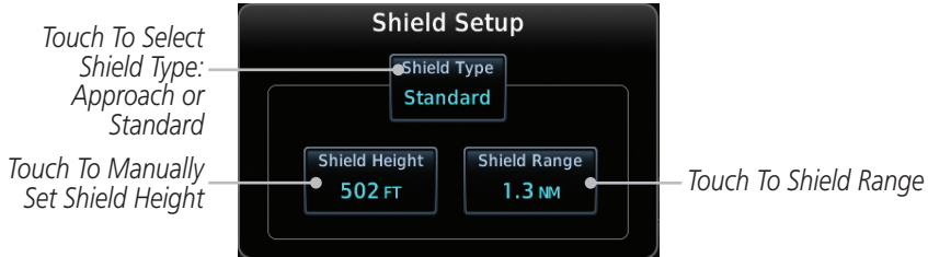
Figure 10-29 TCAD 9900B Shield Setup for En Route, Standard, and Terminal
