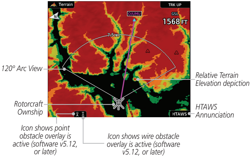
Figure 11-25 Terrain/HTAWS Page
