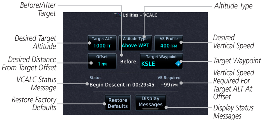
Figure 15-5 VCALC Page
