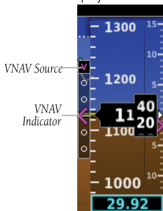
Figure 2-28 VNAV Indicator - PFD
