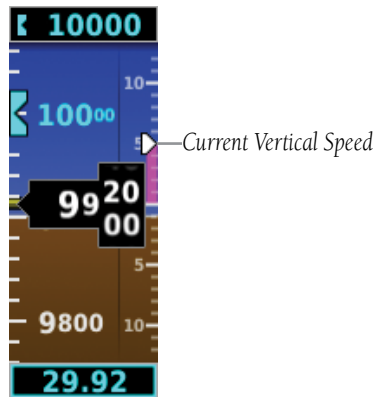
Figure 2-14 Vertical Speed Indicator
