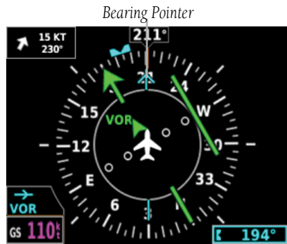
Figure 2-18 VOR Source Bearing Pointer
